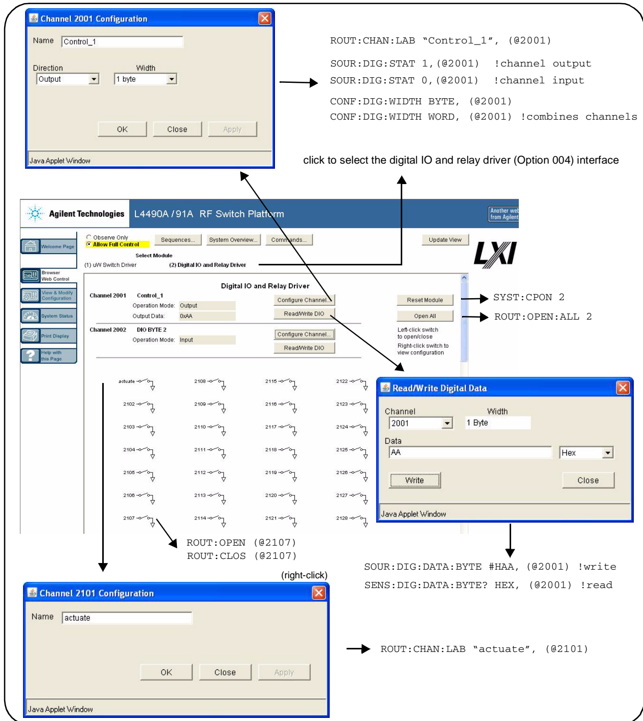
Figure 4-17. L4490A / L4491A Option 004 Web User Interface.
